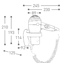
Wall holder with interrupter switch. Hard wired.
